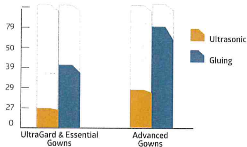
Average Sleeve Seam Tensile Strength (N)
