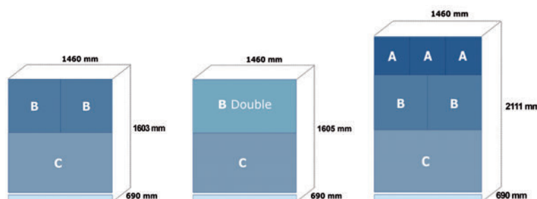
CP003020 - Set of 2 polyester cages : 1C+ 1 Double B stainless steel grid doors + partition + 1 mobile platform
