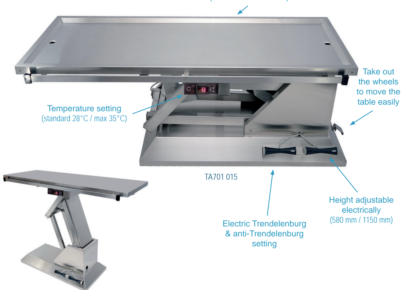
TA701 000 - Heated flat top
